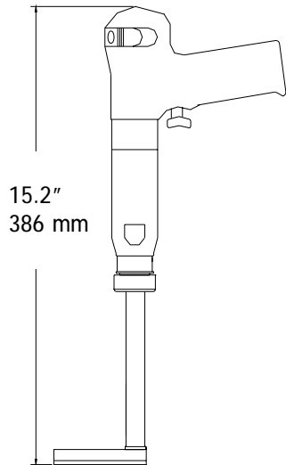
CLECO 8 .45 HP MOTOR 200 R.P.M. REVERSIBLE WEIGHT: 4.4 LBS. 2.00 Kg.
