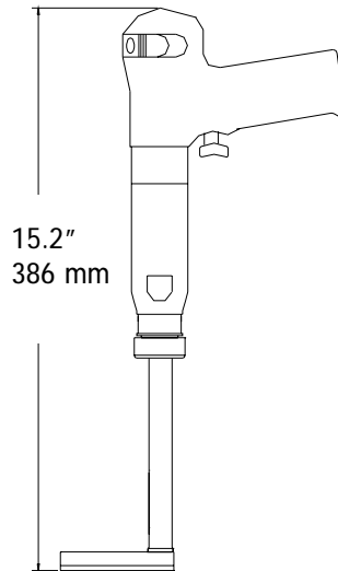
CLECO 8 .45 HP MOTOR 400 R.P.M. REVERSIBLE WEIGHT: 4.4 LBS. 2.00 Kg.
