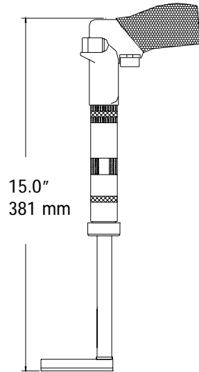
CLECO 5 .33 HP MOTOR 420 R.P.M. REVERSIBLE WEIGHT: 2.8 LBS. 1.27 Kg.
