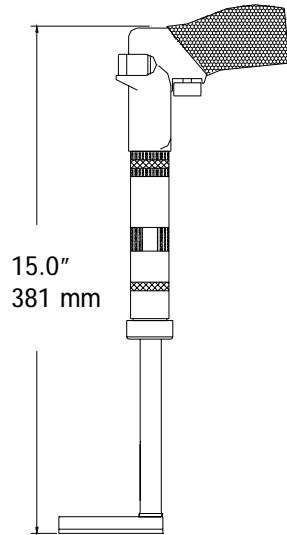
CLECO 5 .33 HP MOTOR 175 R.P.M. REVERSIBLE WEIGHT: 2.8 LBS. 1.27 KG.
