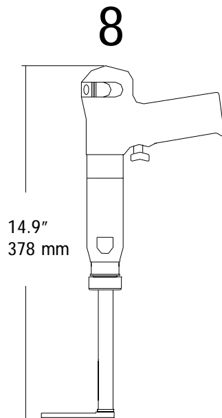
CLECO 8 .45 HP MOTOR 200 R.P.M. REVERSIBLE WEIGHT: 4.2 LBS. 1.90 Kg.
