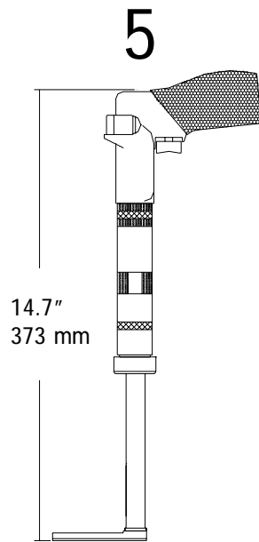
CLECO 5 .33 HP MOTOR 175 R.P.M. REVERSIBLE WEIGHT: 2.6 LBS. 1.18 Kg.
