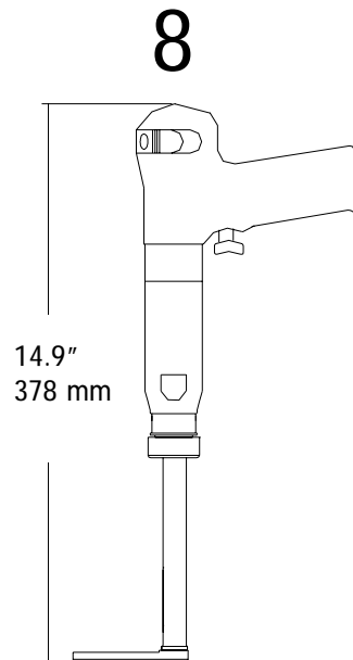
CLECO 8 .45 HP MOTOR 400 R.P.M. REVERSIBLE WEIGHT: 4.2 LBS. 1.90 Kg.
